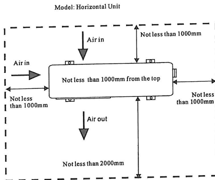
Free space requirement for the horizontal heat pump
